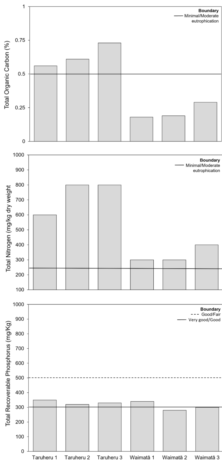
Figure 12. Sediment total organic carbon (TOC), total nitrogen (TN), and total recoverable phosphorus (TRP) content at the Taruheru and Waimatā sites. Top and middle: Horizontal lines indicate TOC and TN levels for minimal to moderate eutrophication based on the Estuary Trophic Index (Robertson et al. 2016b). Bottom: Guidelines for good / fair health are based on Robertson and Stevens (2010).
