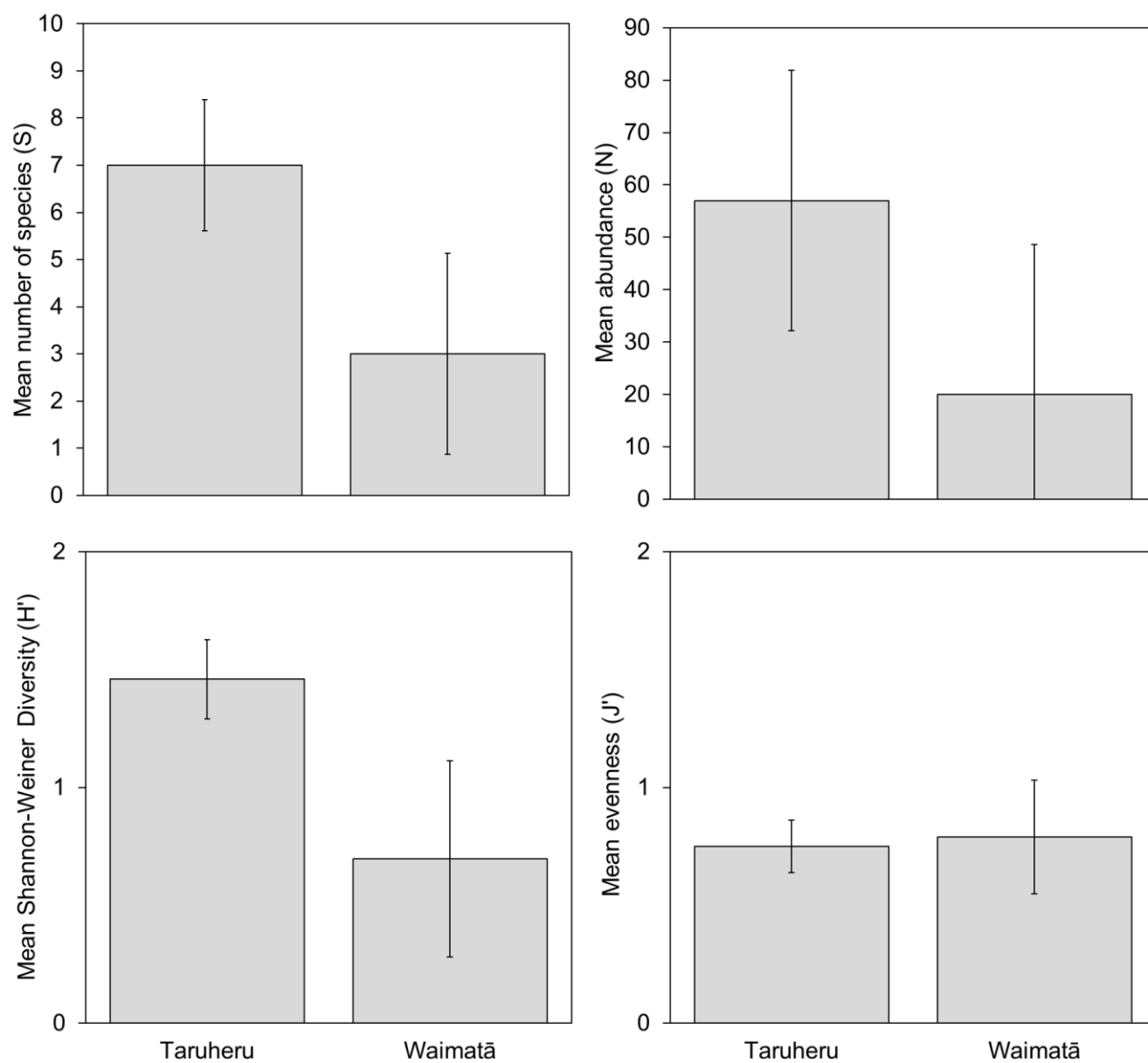
Figure 16. Community indices for the Taruheru and Waimatā fine-scale sites in Tūranganui Estuary. Number of macroinvertebrate species ( S ) and diversity ( H' ; left) and infauna abundance ( N ) and evenness ( J' ; right).
