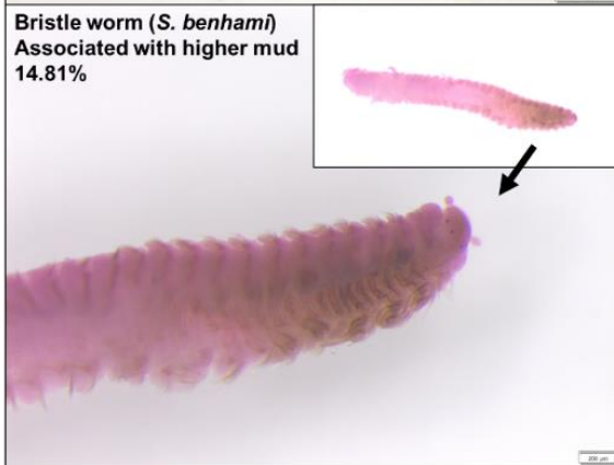
Figure 26. Indicator species contributing to similarity (%; SIMPER) among samples within the Taruheru and Waimatā sites in Tūranganui Estuary (refer to Table 12). Infauna at the Taruheru site were dominated by more mud-tolerant species, whereas infauna at the Waimatā site were dominated by mud-sensitive species. Image credits: MacLean Marine Identifiers.
