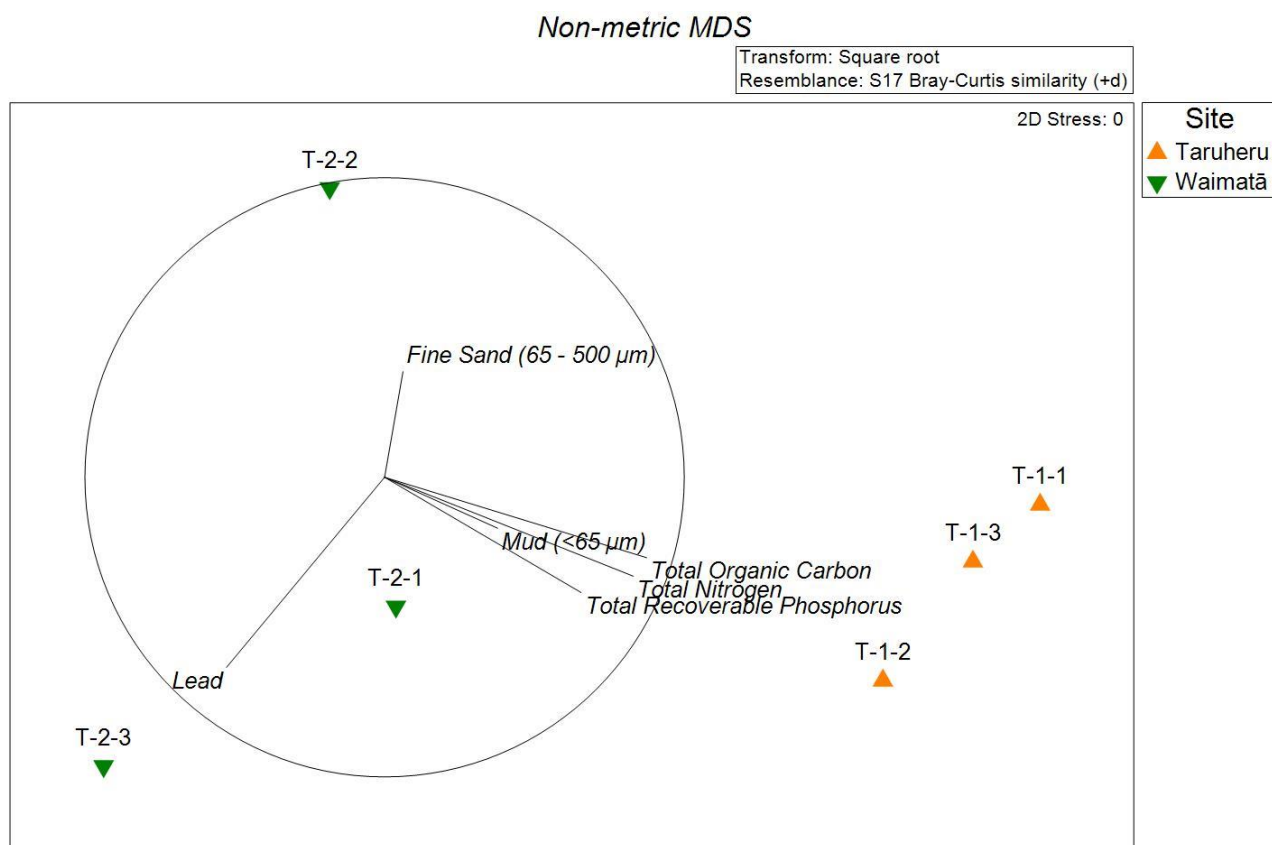
Figure 21. Differences in macroinvertebrate communities are typically explained by variations in sediment composition (sand and fine sand), nutrient content and lead content. Each symbol represents a macroinvertebrate community sampled from each plot of the Taruheru and Waimatā sites in Tūranganui Estuary. Note that symbols that appear closer together represent communities that are more similar than those spread farther apart.
