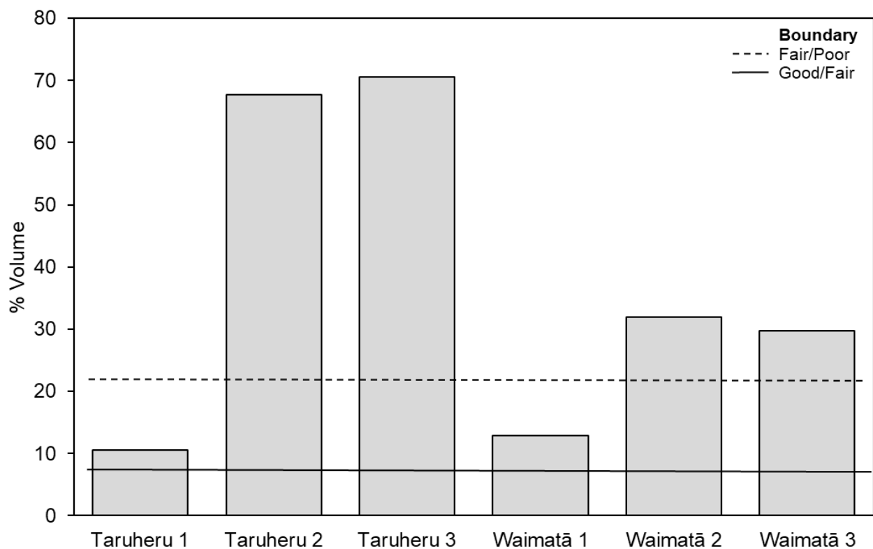
Figure 9. Sediment mud (< 63 µm) content (% volume) at the Taruheru and Waimatā sites in Tūranganui Estuary. Horizontal lines indicate poor, fair and good health based on LAWA guidelines.
